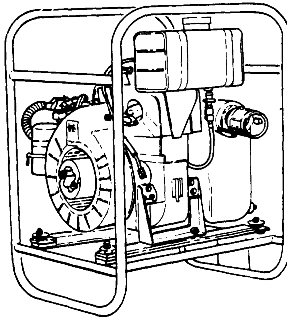
Figure 1-8. 125 GPM Pump Assembly
