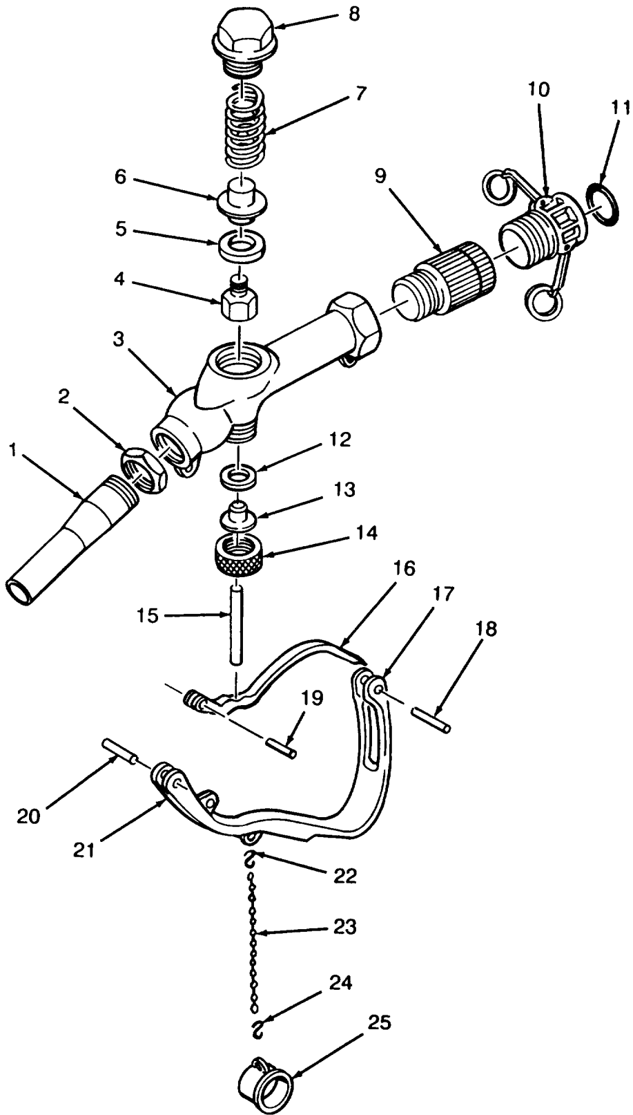
Distribution Nozzle
