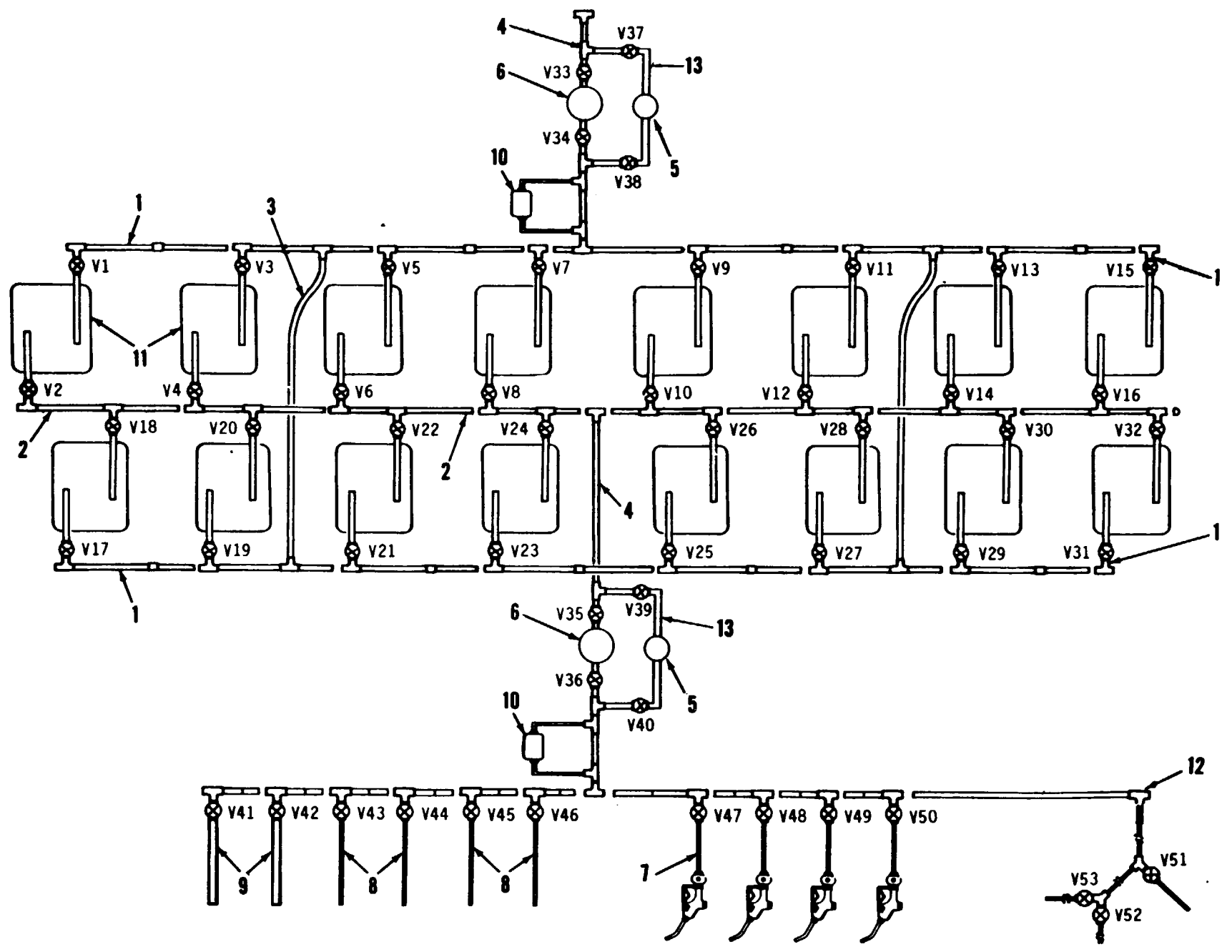
Figure 1-3. 300K Water Distribution System
