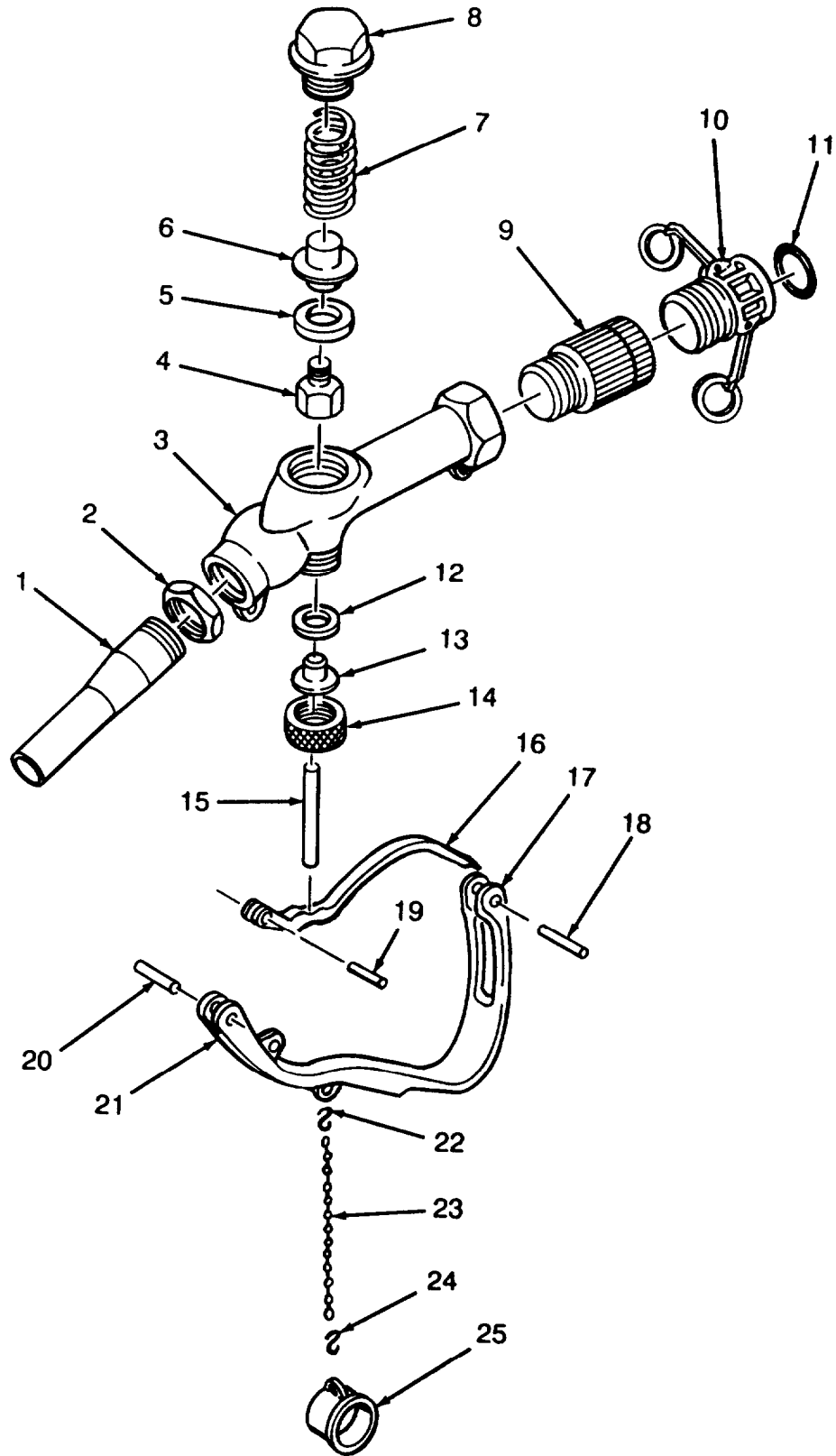
Distribution Nozzle
